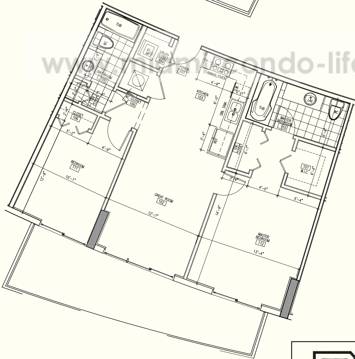
UNIT D1 FLOORPLAN - LEVELS 5-14
