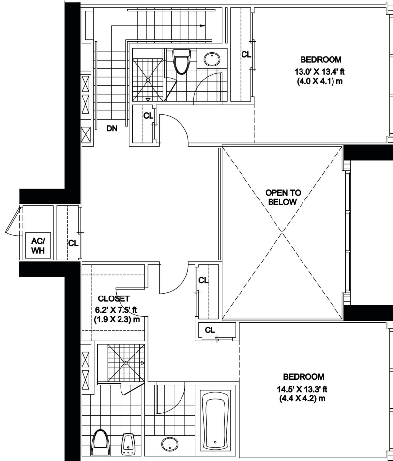
UPPER LEVEL
